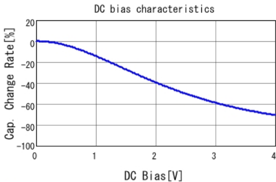
■ GRM21BR60G476ME01 C-DC bias capchange, 25.0degC, AC0.
