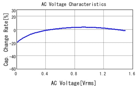
■ GRM21BR60G476ME01 C-AC Voltage capchange, DCOV, 25.0d
