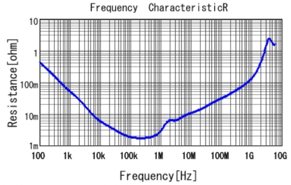
■ GRM21BR60G476ME01 R DCOV, 25degC
