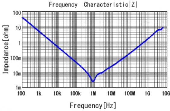
■ GRM21BR60G476ME01 |Z| DCOV, 25degC
