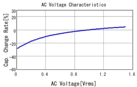
■ GRM21BC71E106KE11 C-AC Voltage capchange, DC0V, 25.0d
