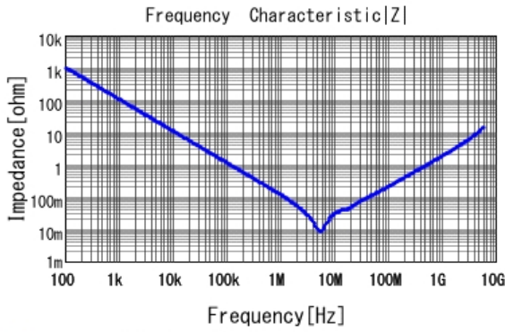
■ GRM188R71A225KE15 |Z| DCOV, 25degC
