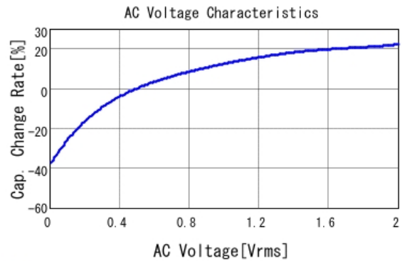
■ GRM188R71A225KE15 C-AC Voltage capchange, DCOV, 25.0d
