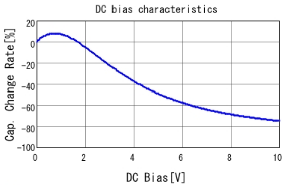
■ GRM188R71A225KE15 C-DC bias capchange, 25.0degC, AC0.
