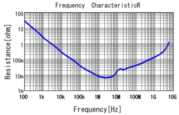
■ GRM188R71A225KE15 R DCOV, 25degC
