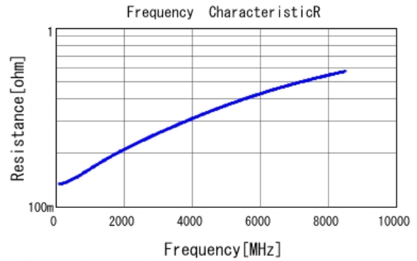
■ GRM0225C1H9R1WA03 R DCOV, 25degC
