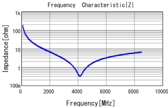
■ GRM0225C1H9R1WA03 |Z| DCOV, 25degC
