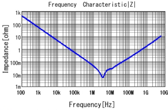
■ GRM188R6YA475KE15 |Z| DCOV, 25degC
