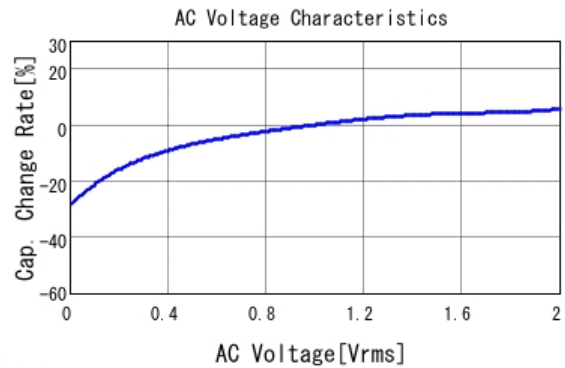
■ GRM188R6YA475KE15 C-AC Voltage capchange, DCOV, 25.0d
