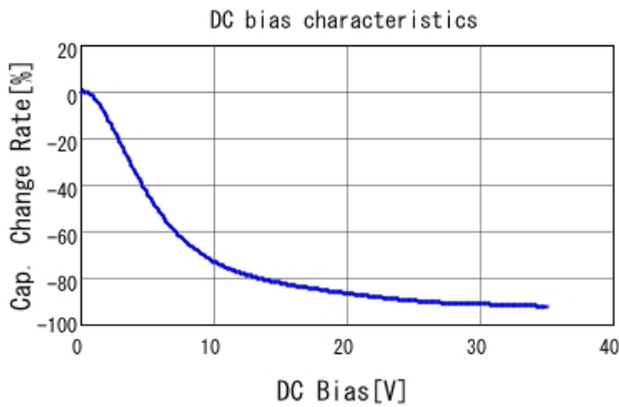
■ GRM188R6YA475KE15 C-DC bias capchange, 25.0degC, AC1V
