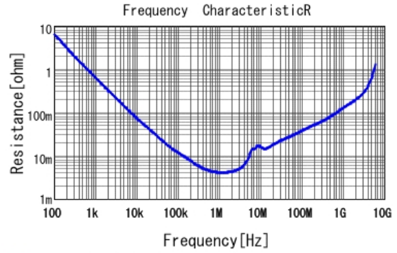
■ GRM188R6YA475KE15 R DCOV, 25degC
