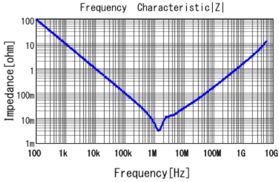
■ GRM21BD71A226ME44 |Z| DCOV, 25degC
