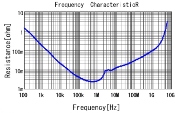
■ GRM21BD71A226ME44 R DCOV, 25degC
