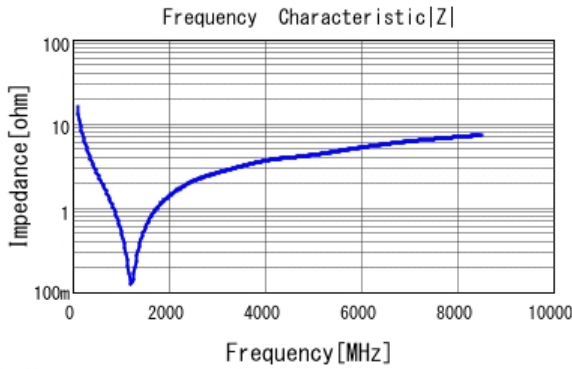
■ GRM0225CYA101JA02 |Z| DCOV, 25degC
