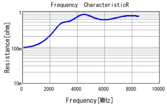
■ GRM0225CYA101JA02 R DCOV, 25degC
