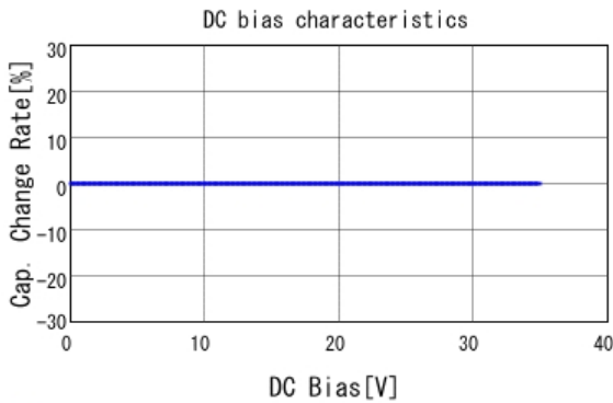
■ GRM0225CYA101JA02 C-DC bias capchange, 25.0degC, AC1V
