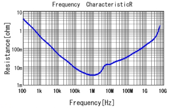
■ GRM188C81A106MA73 R DCOV, 25degC
