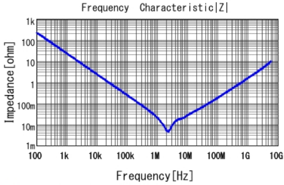
■ GRM188C81A106MA73 |Z| DCOV, 25degC
