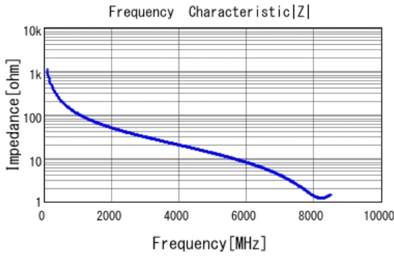
■ GRM0335C1H1R5BA01 |Z| DC0V, 25degC
