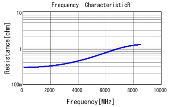
■ GRM0335C1H1R5BA01 R DC0V, 25degC
