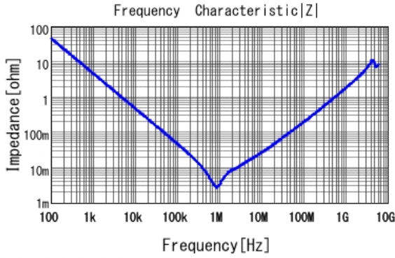
■ GRM21BC80G476ME15 |Z| DCOV, 25degC
