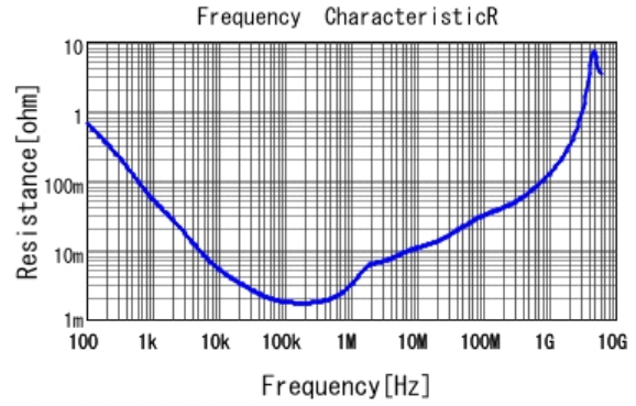
■ GRM21BC80G476ME15 R DCOV, 25degC
