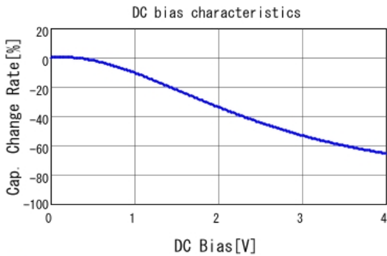
■ GRM21BC80G476ME15 C-DC bias capchange, 25.0degC, AC0.
