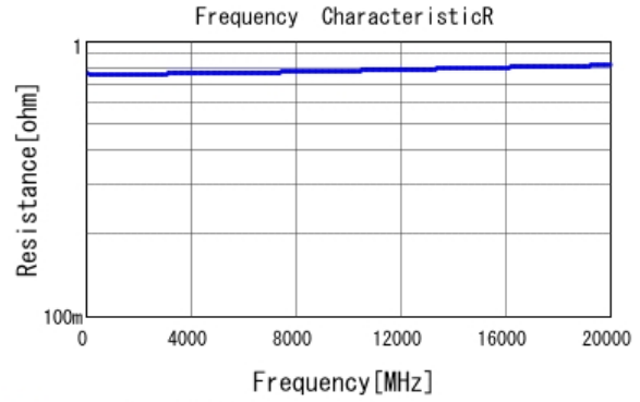
■ GRM0225C1HR30WA03 R DCOV, 25degC
