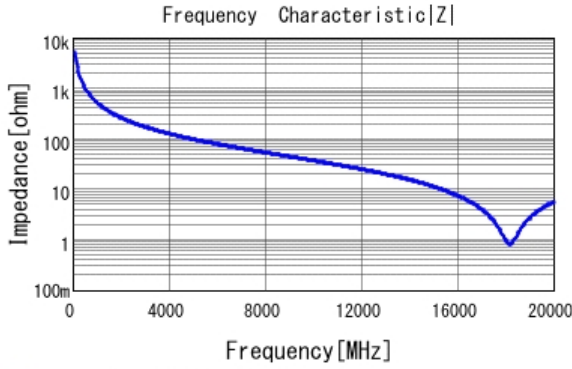
■ GRM0225C1HR30WA03 |Z| DCOV, 25degC
