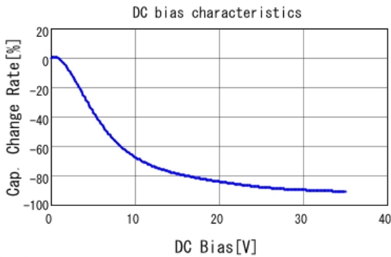
■ GRM21BC8YA106KE11 C-DC bias capchange, 25.0degC, AC1V
