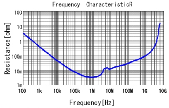
■ GRM21BC8YA106KE11 R DCOV, 25degC
