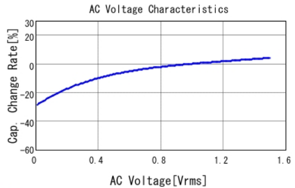
■ GRM21BC8YA106KE11 C-AC Voltage capchange, DCOV, 25.0d
