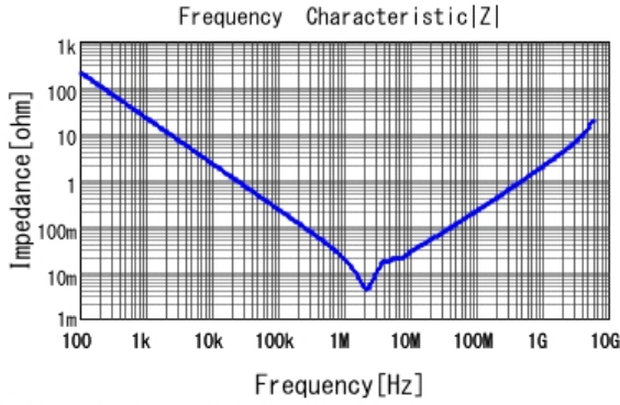
■ GRM21BC8YA106KE11 |Z| DCOV, 25degC
