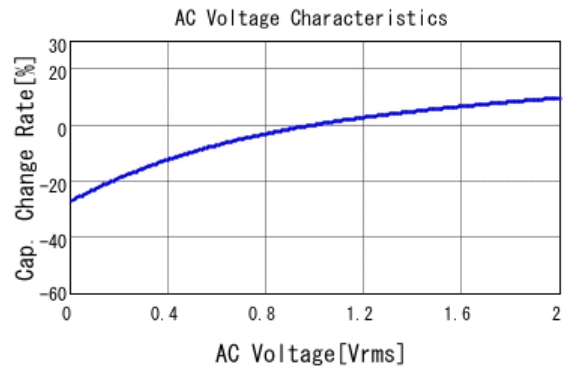
■ GRM21BC71E475KE11 C-AC Voltage capchange, DCOV, 25.0d
