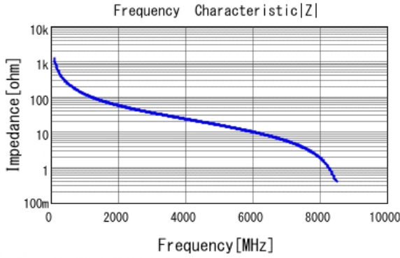
■ GJM0335C1E1R3BB01 |Z| DC0V, 25degC
