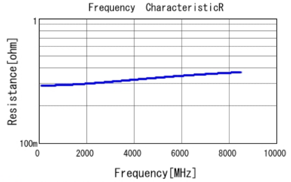
■ GJM0335C1E1R3BB01 R DC0V, 25degC
