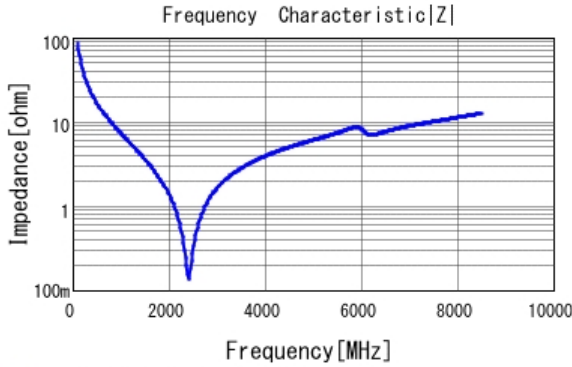
■ GJM0335C1E180JB01 |Z| DC0V, 25degC
