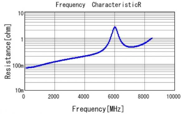
■ GJM0335C1E180JB01 R DC0V, 25degC
