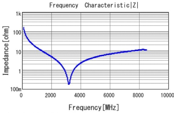
■ GJM0335C1E100JB01 |Z| DC0V, 25degC
