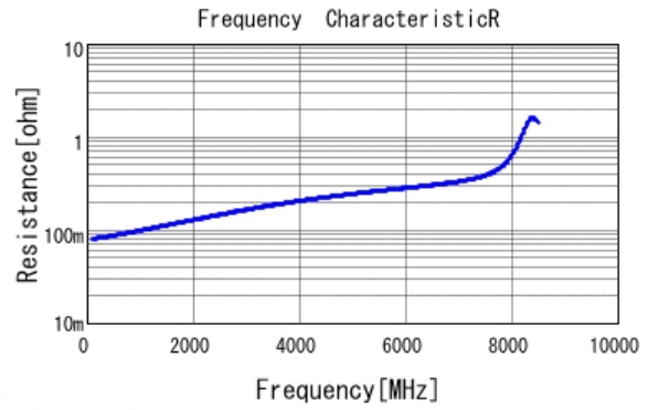
■ GJM0335C1E100JB01 R DC0V, 25degC
