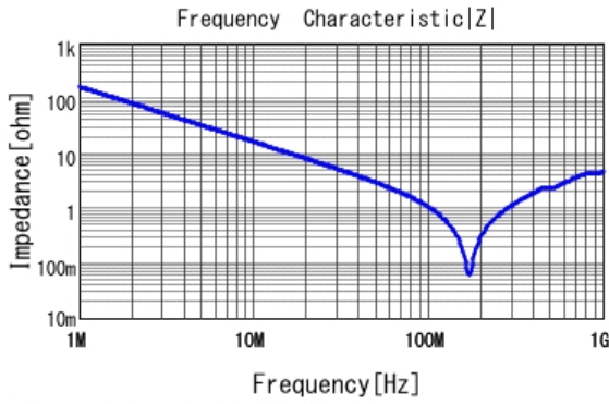
■ GCM31A5C2J102JX01 |Z| DC0V, 25degC
