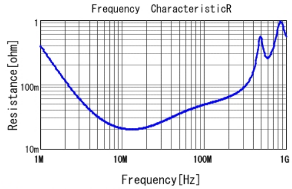
■ GCM31A5C2J102JX01 R DC0V, 25degC
