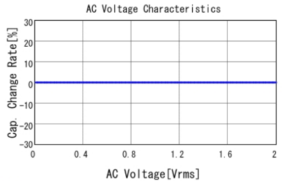
■ GCM3195C2A682JA16 C-AC Voltage capchange, DCOV, 25.0d
