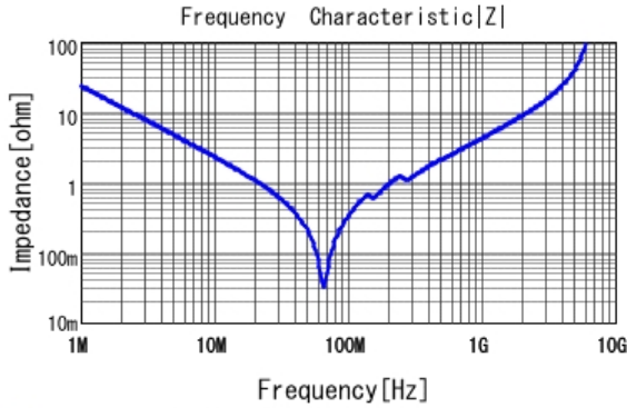
■ GCM3195C2A682JA16 |Z| DCOV, 25degC
