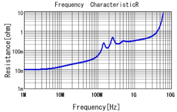
■ GCM3195C2A682JA16 R DCOV, 25degC
