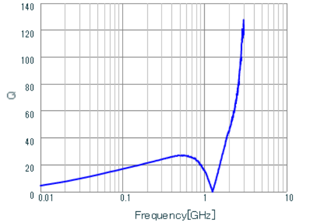
LQG15WZR11J02 Q.
