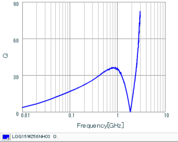
Q-Frequency Characteristics
