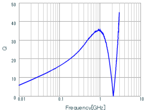
Q-Frequency Characteristics
