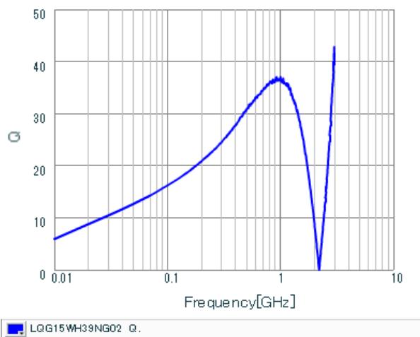
Q-Frequency Characteristics
