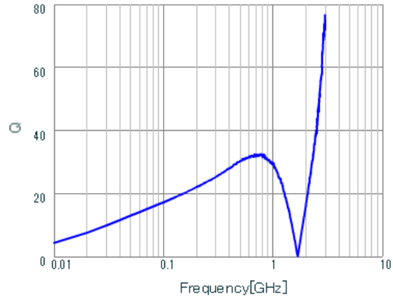
LQG15WH68NG02 Q.
