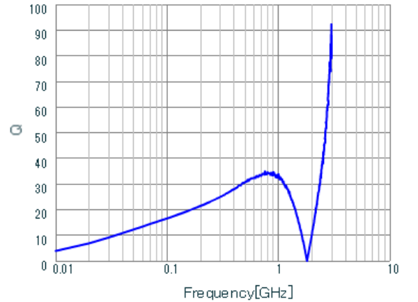
Q-Frequency Characteristics
