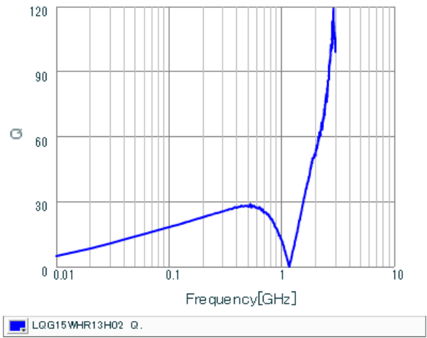
Q-Frequency Characteristics
