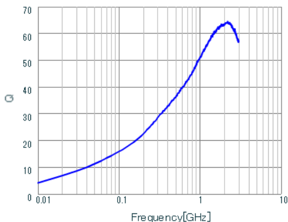
Q-Frequency Characteristics
