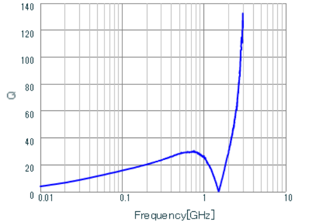
LQG15WH75NG02 Q.
