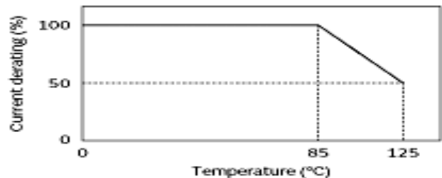
Derating of Rated Current
