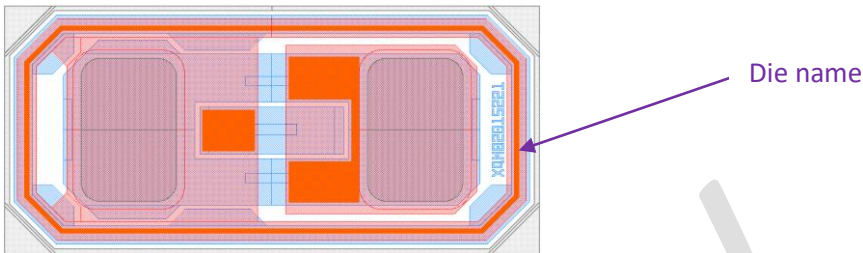
Figure 6 – Layout view
