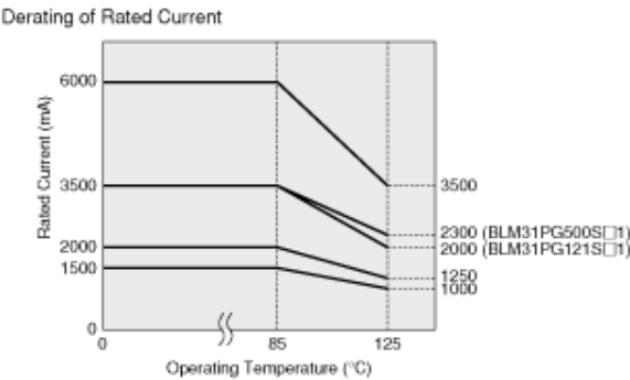
Derating of Rated Current
