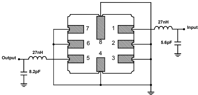
Matching Circuit to 50Ω
