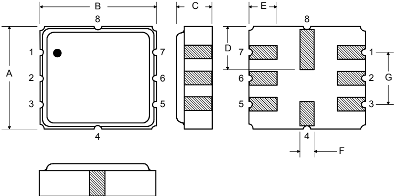
Case Dimensions
