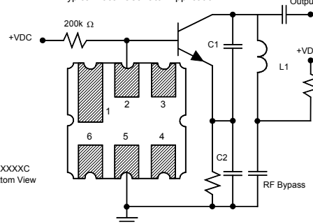
Typical Local Oscillator Application
