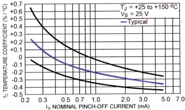
FIGURE 2 – TEMPERATURE COEFFICIENT
