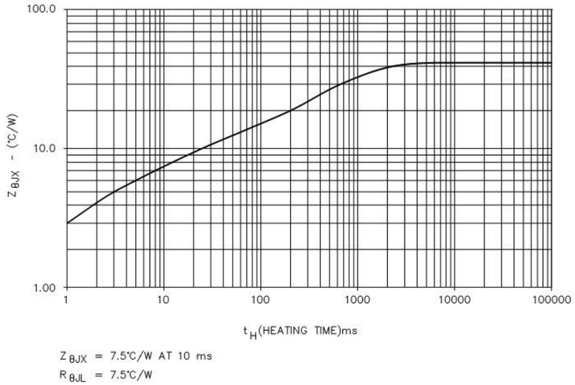
FIGURE 9. Thermal impedance curve for 1N6485 through 1N6491 and 1N4460 through 1N4461.
