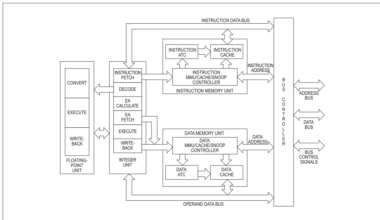
FIGURE 1 – BLOCK DIAGRAM
