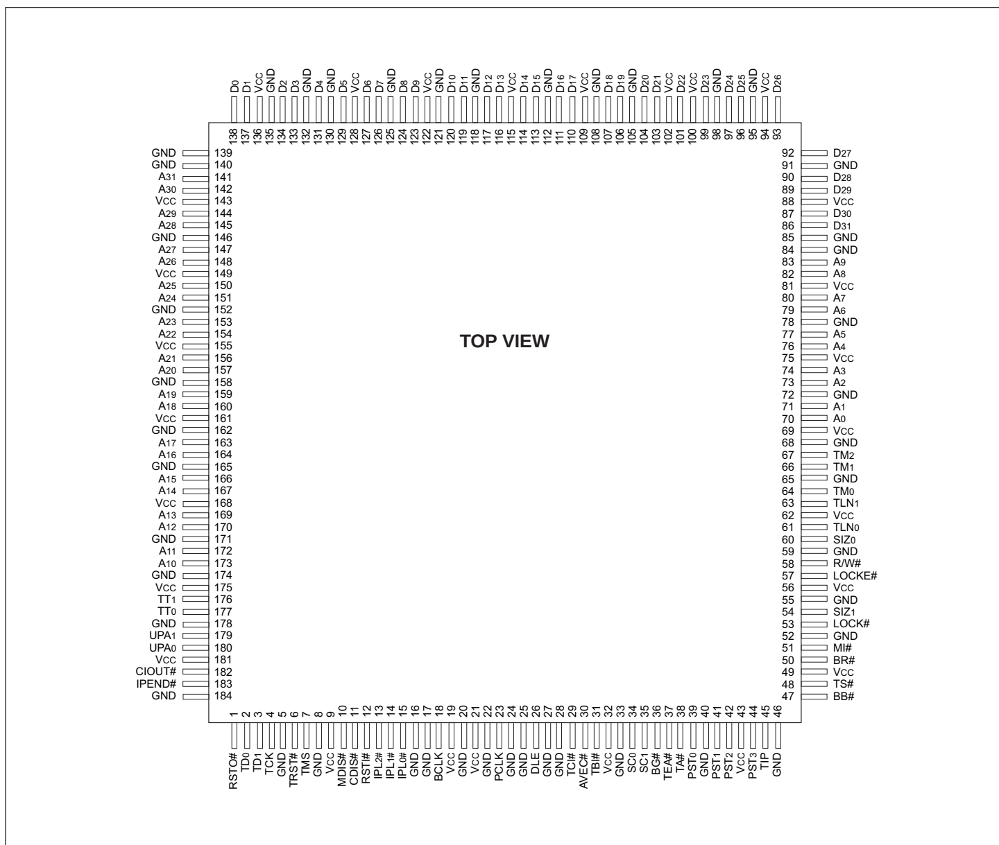
FIGURE 2 – PIN CONFIGURATION FOR WC32P040-XXM, CQFP (Q4)
