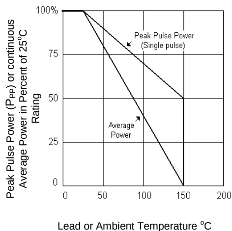
FIGURE 3 Derating Curve
