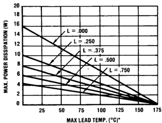
FIGURE 6 MAXIMUM LEAD TEMP. vs. PD
