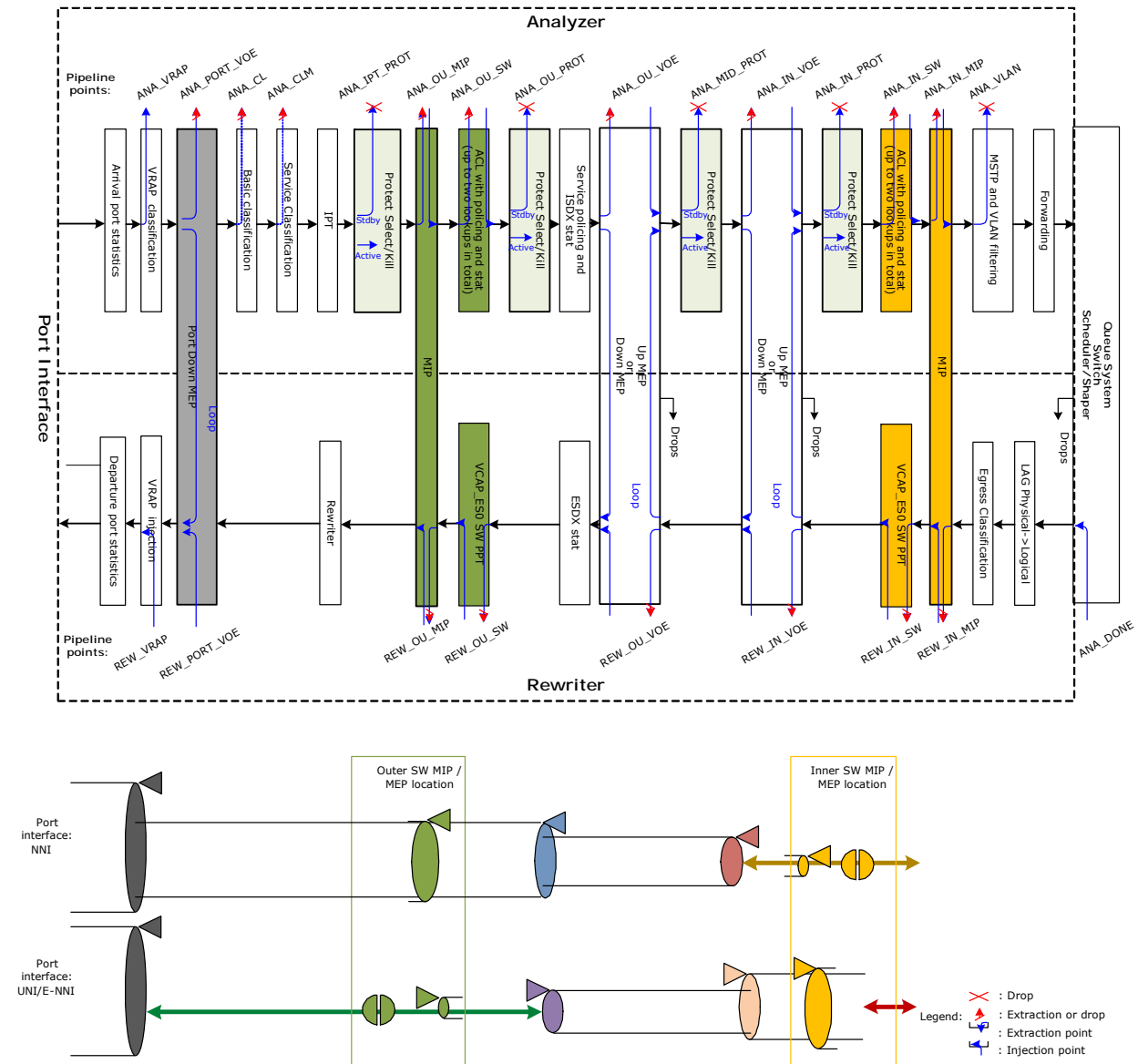
Figure 21 • Processing Flow
