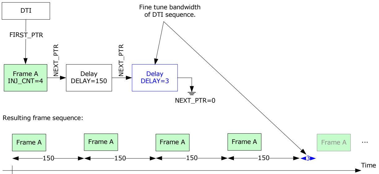
Figure 99 • Fine Tuning Bandwidth of DTI Sequence
