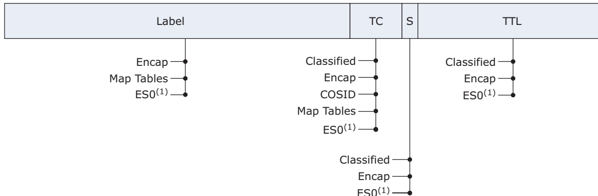
Figure 110 • MPLS Remarking
