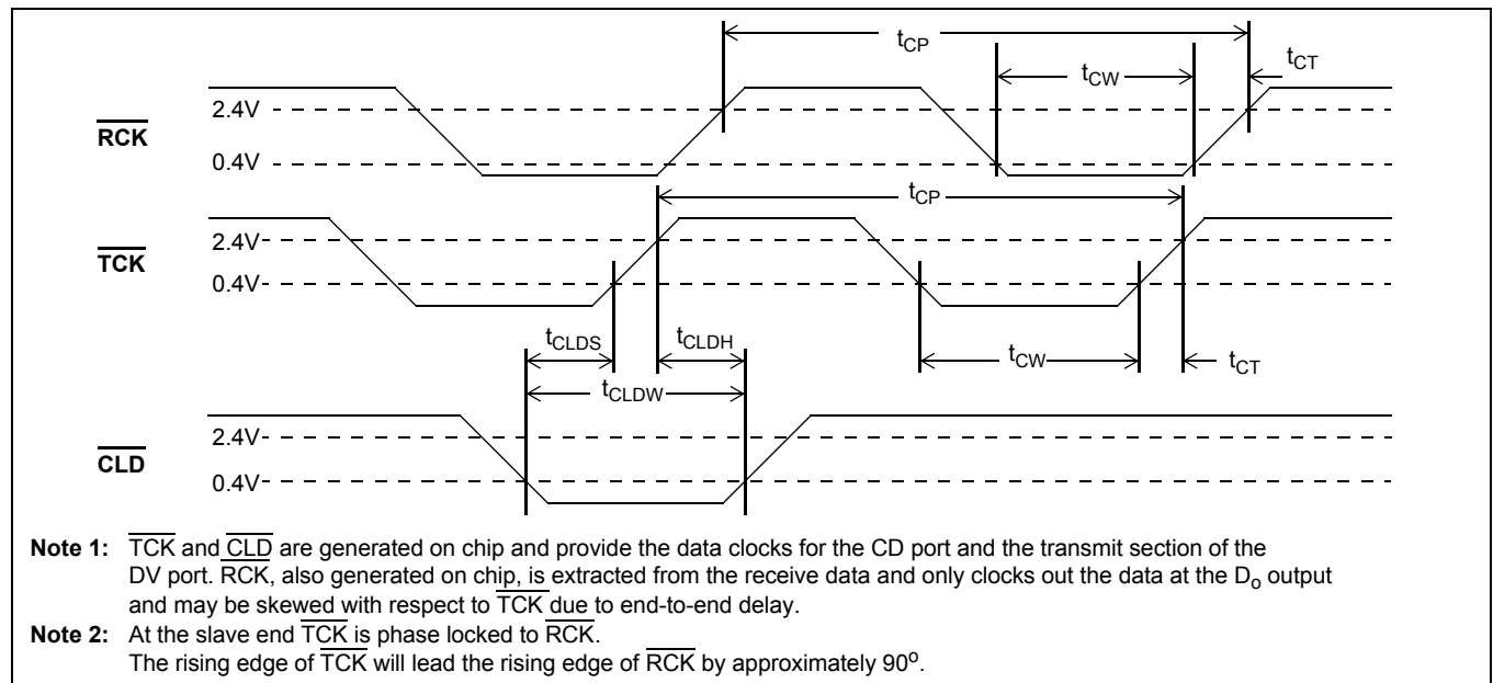
Figure 18 - \overline{\text{RCK}} , \overline{\text{TCK}} & \overline{\text{CLD}} Timing For MOD Mode
