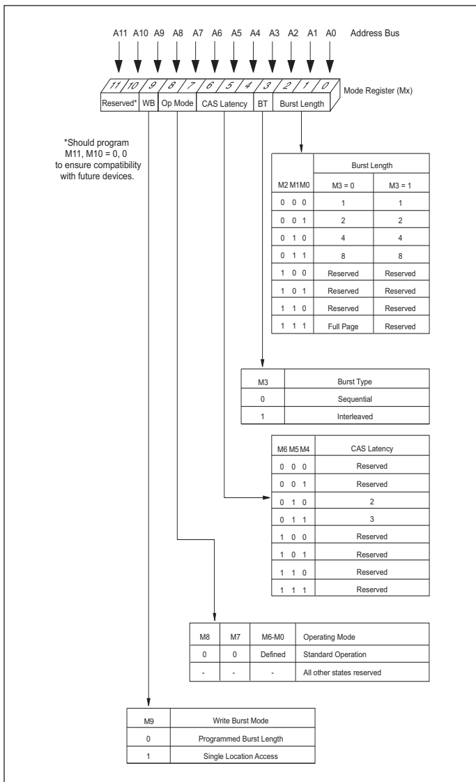
FIGURE 2 – MODE REGISTER DEFINITION
