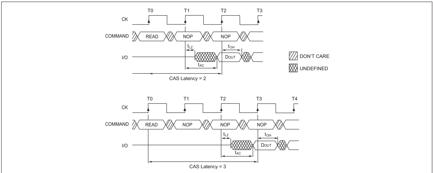
FIGURE 3 – CAS LATENCY
