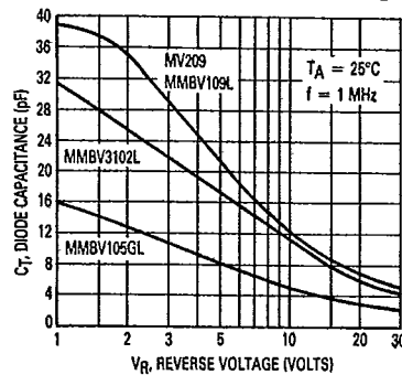
Diode Capacitance versus Reverse Voltage
