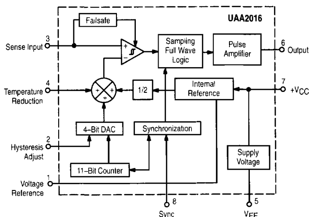
Representative Block Diagram
