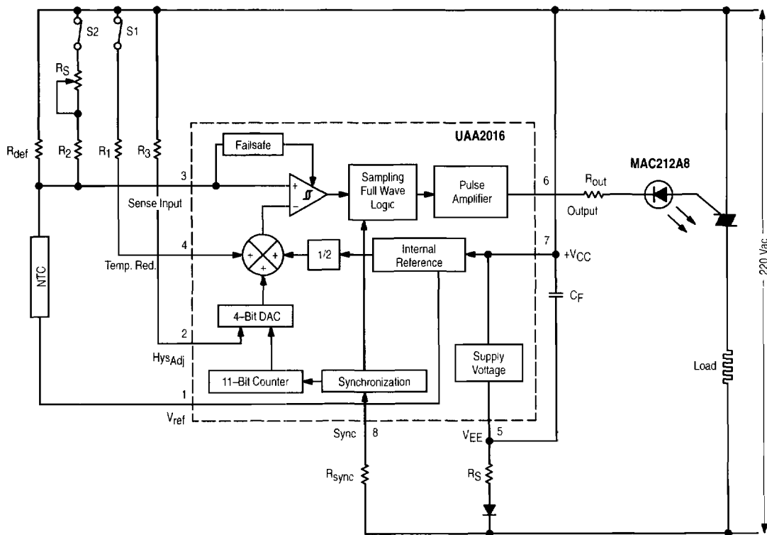
Figure 1. Application Schematic
