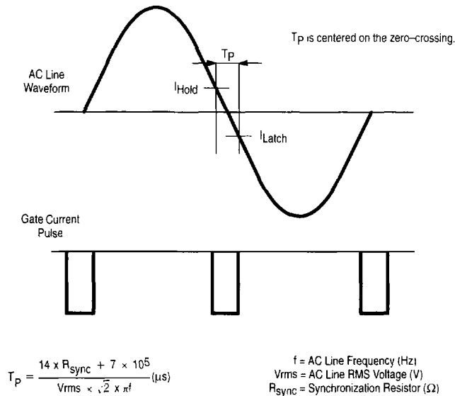
Figure 3. Zero Voltage Technique
