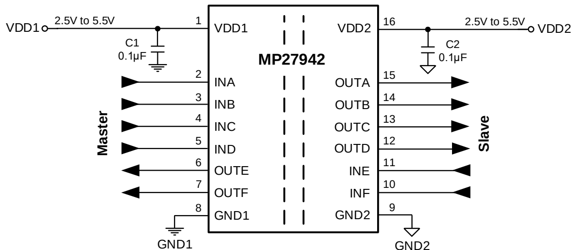
Figure 9: Typical Application Circuit (6 Channels, Channel Direction: 4 Forward and 2 Reverse, Isolated Interface)
