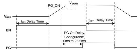
Figure 17: Power Good On/Off Sequence
