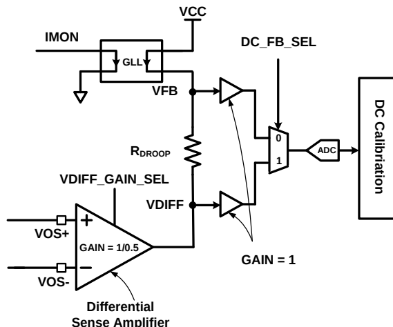
Figure 12: DC Loop Gain Selection
