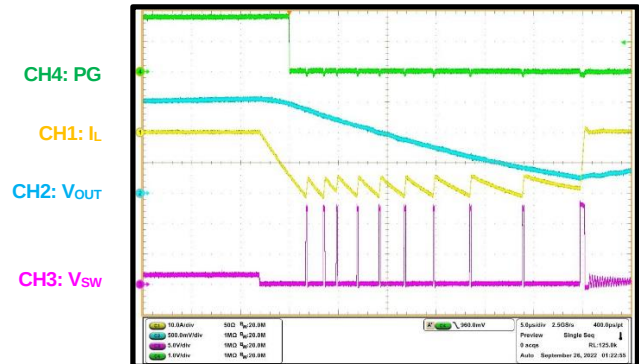
OVP/NOCP OVP level = 130% of VID, NOCP = -20A, OVP trigger delay = 1μs, hiccup mode
