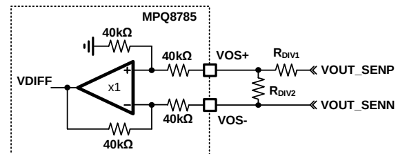
Figure 13: Output Divider with Remote Sense
