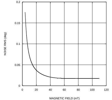
RMS Noise
