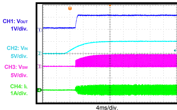
V_{IN} Power-Up
