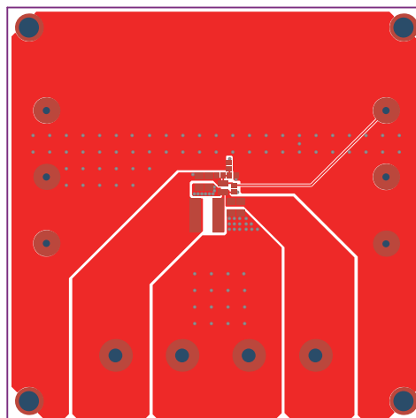
Figure 3: Top Layer
