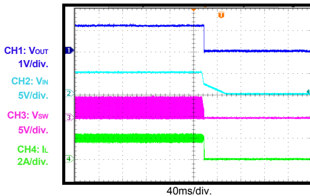
V_{IN} Shutdown
