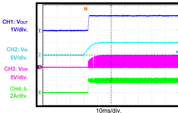
V_{IN} Power-Up
