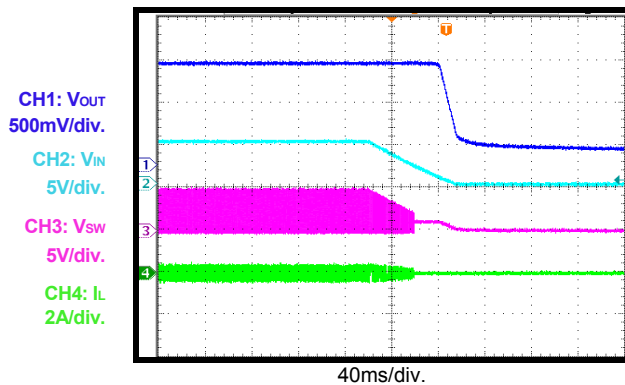
V_{IN} Shutdown
