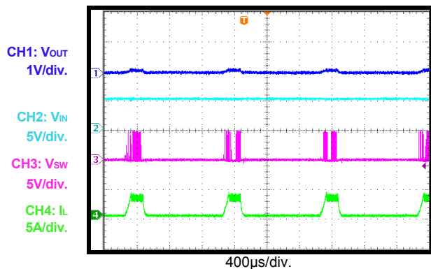
Short-Circuit State
