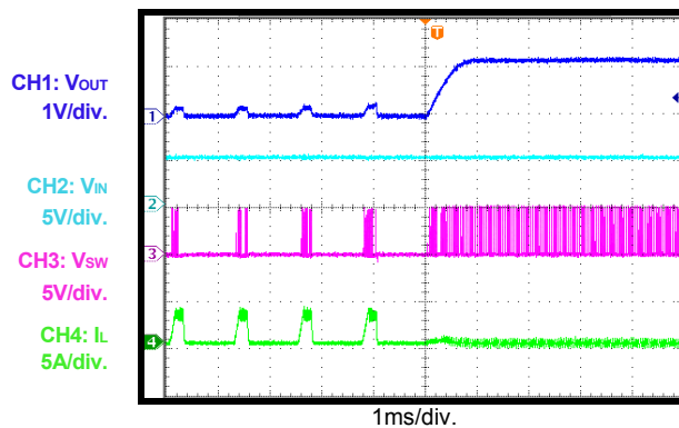
Short-Circuit Recovery
