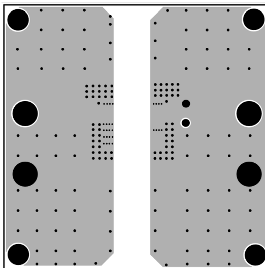
Figure 5: Bottom Layer
