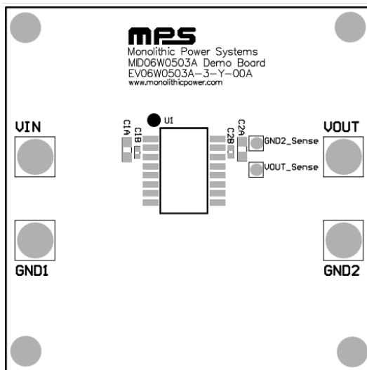
Figure 3: Top Silk
