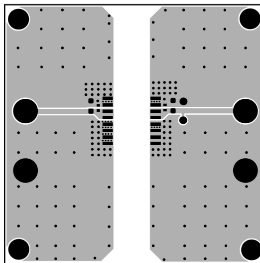
Figure 4: Top Layer
