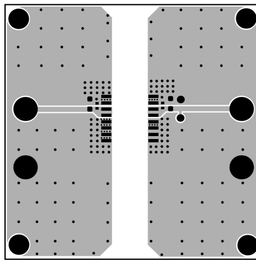
Figure 2: Top Layer
