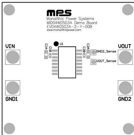
Figure 1: Top Silk
