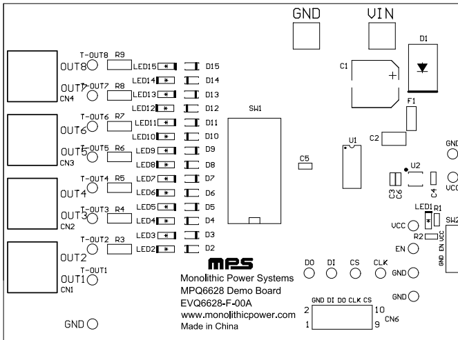
Figure 4: Top Silk
