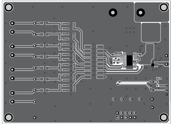
Figure 5: Top Layer
