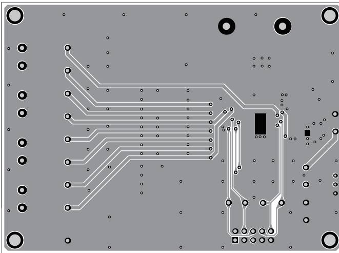
Figure 6: Bottom Layer
