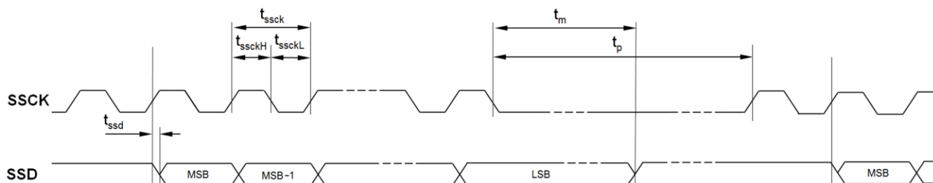
Figure 15: SSI Timing
