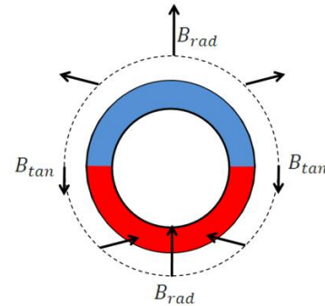
Figure 19: Side-Shaft Field
