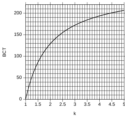
Figure 20: Relation between the k Ratio and the Optimum BCT to Recover Linearity
